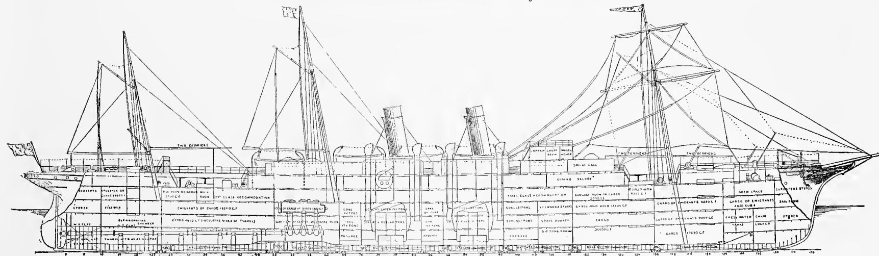
GENERAL PLAN OF STEAMSHIP EMPRESS OF JAPAN.
